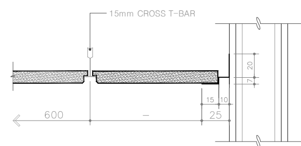
7 SECTION DETAIL 2 SCALE : NONE
