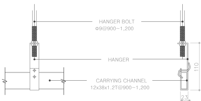
5 SECTION DETAIL 1 SCALE : NONE
