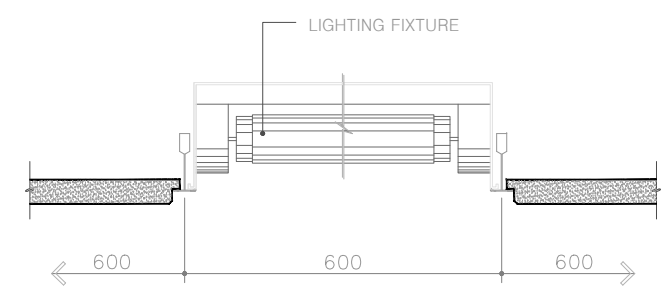
3 "B" SECTION DETAIL SCALE : NONE
