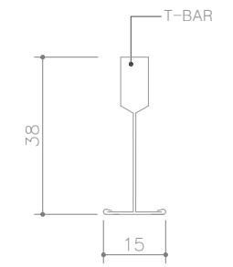
6 SECTION DETAIL 1 SCALE : NONE
